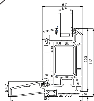
Alu bunnkarm
