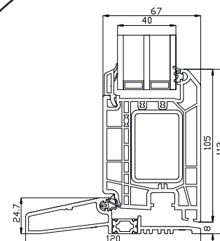
Alu bunnkarm
