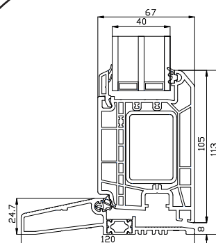
Alu bunnkarm
